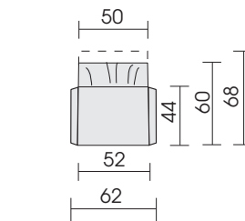
Chair with armrest functional back C53
