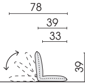
Side view type 572
